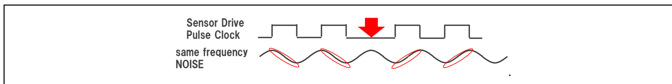
Figure 3-2 Periodic Noise Desynchronization by Random Phase Shift Function (image)
