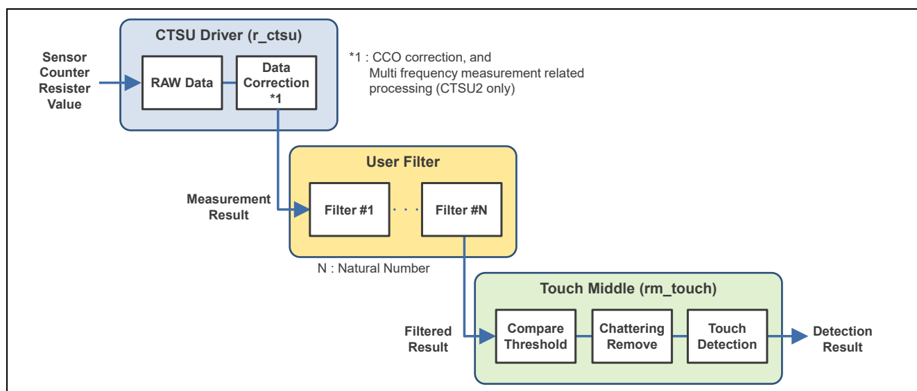
Figure 5-1 Data Flow Through Touch Detection
