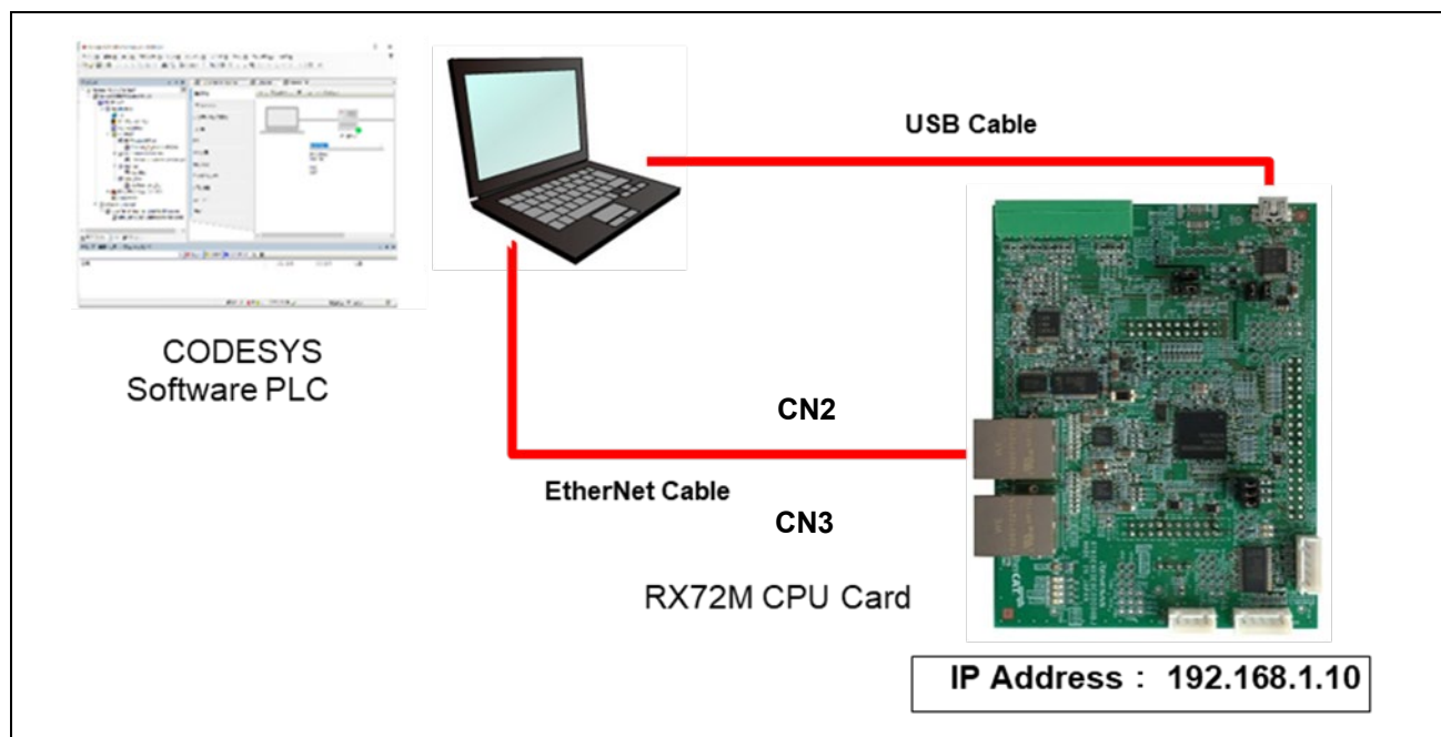
Figure 5.1 Connection configuration
